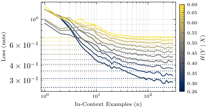
In-Context Learning Loss for Qwen-2.5 (7B)
